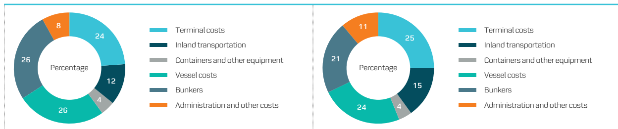
Distribution of container shipping unit costs
